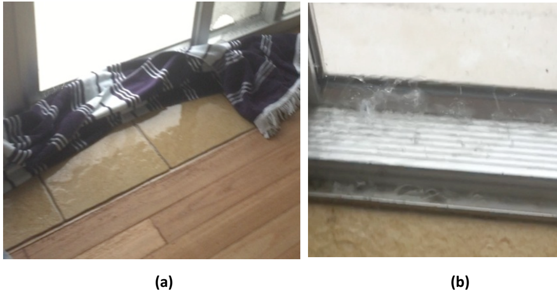
Figure 1 (a) Towels placed in front of large windward wall windows to control large amounts of water, and (b) water spraying into living room from under the door (CTS TR63)
